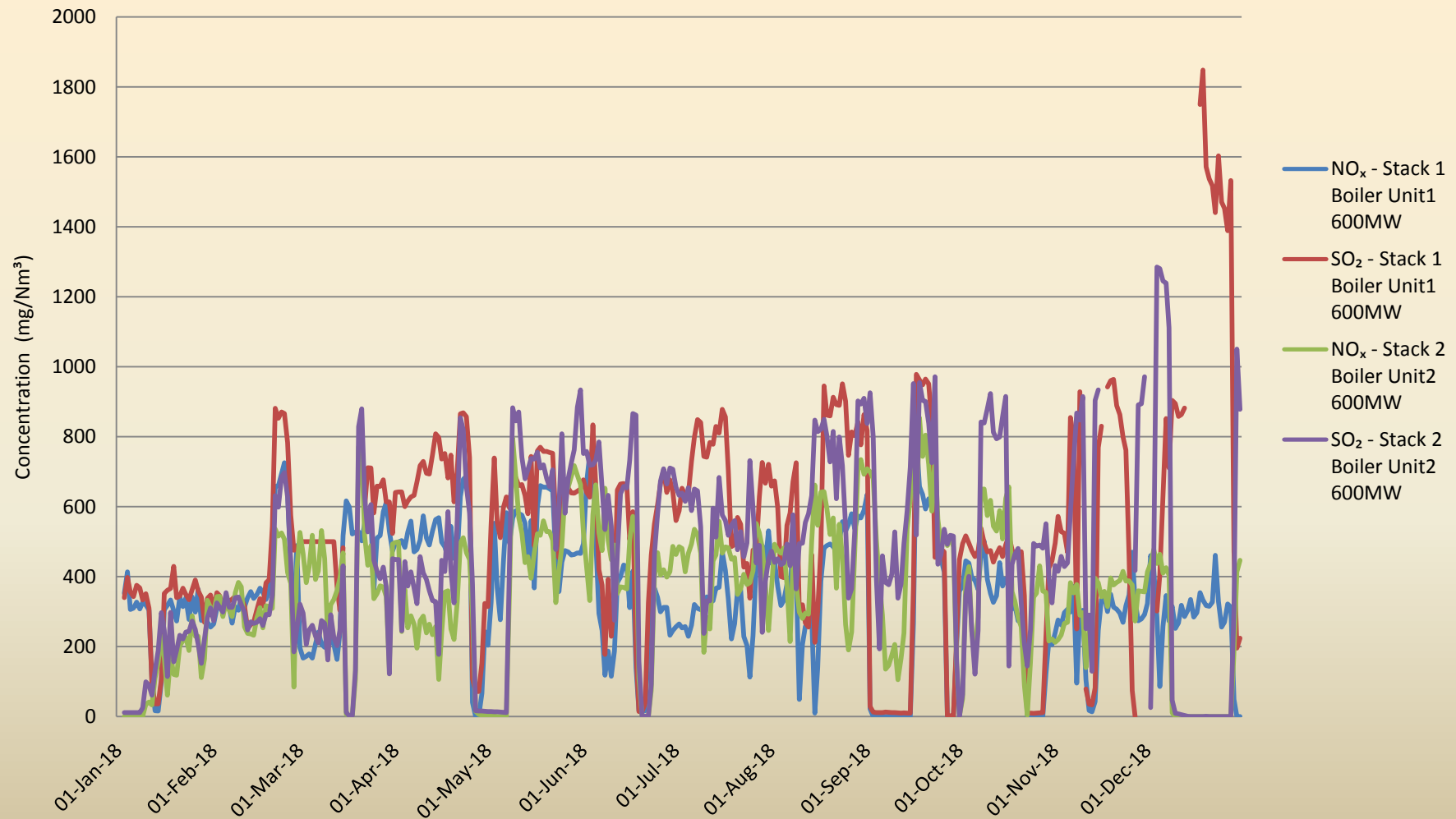
Annual Emission Trend of Gaseous in M/s. M.B. Power (M.P.) Limited, Dist. Anuppur (M.P.)
